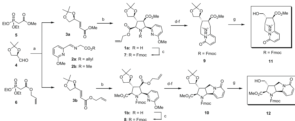
Scheme 1. Reagents and conditions: (a) NaH, THF, 5 or 6 ; (b) 3a/2a or 3b/2b , AgOAc, DBU, toluene, -78^{\circ}\text{C} , 86–90%; (c) FmocCl, DIEA DCM, 81–90%; (d) Pd(PPh 3 ) 4 , PhMeNH, THF, 82–99%; (e) BOP, NaBH 4 , THF, 70–75%; (f) (i) MsCl, Et 3 N; (ii) toluene, reflux, 70–74%; (g) (i) HCl, THF, H 2 O; (ii) NaIO 4 ; (iii) NaBH 4 , 76–78%.
