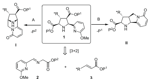
Figure 2. Cyclization strategy to form pyridone scaffolds I and II .
