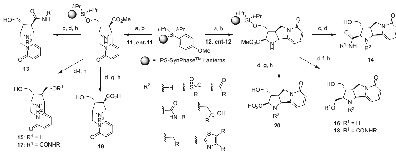
Scheme 2. Reagents and conditions: (a) (i) TFOH (6.0 equiv), DCM; (ii) 11 , ent-11 , 12 or ent-12 (1.2 equiv), 2,6-lutidine (9.0 equiv), DCM, rt, 24 h; (b) 20% piperidine, DMF, rt, 30 min; (c) AlMe 3 (15 equiv), amine (20 equiv), toluene, 40 ^{\circ}\text{C} , 3 d; (d) RSO 2 Cl (20 equiv), 2,6-lutidine (25 equiv) DCM, rt, 24 h; RNC(15 equiv), DCM, rt, 24 h; RCOCl (10 equiv), 2,6-lutidine (15 equiv), DCM, rt, 24 h; epoxide (20 equiv), LiClO 4 (20 equiv), i -propanol, 70 ^{\circ}\text{C} , 1–3 d; RCHO (20 equiv), Na(OAc) 3 BH (22 equiv), 2% AcOH, DMF, rt, 3 d; FmocNCS (5 equiv), rt, 24 h then 20% piperidine, DMF, rt, 30 min then RCOCH 2 Br (10 equiv), rt, 24 h; (e) LiBH 4 (5 equiv), THF, rt, 1–2 d; (f) RNC(15 equiv), toluene, 40 ^{\circ}\text{C} , 24 h; (g) LiOH (10 equiv), THF, MeOH, H 2 O, rt, 24 h; (h) (i) 15% HF/pyridine, THF, rt, 2 h; (ii) TMSOMe, 10 min.
