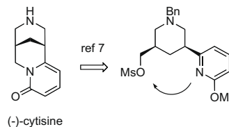
Figure 1. Retrosynthesis of the natural product (–)-cytosine.
